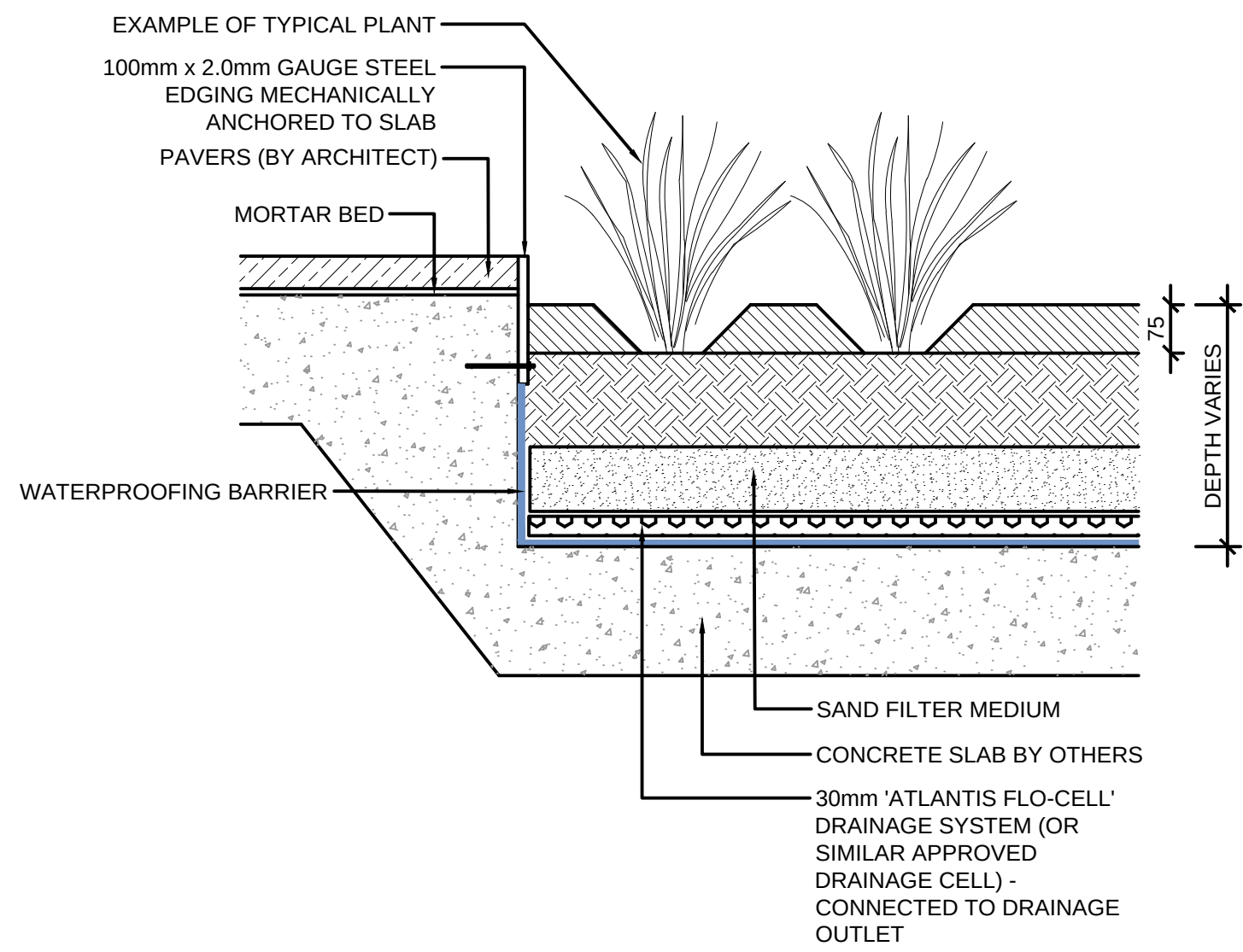
PLANTING ADJACENT PAVING 1:10@A1
