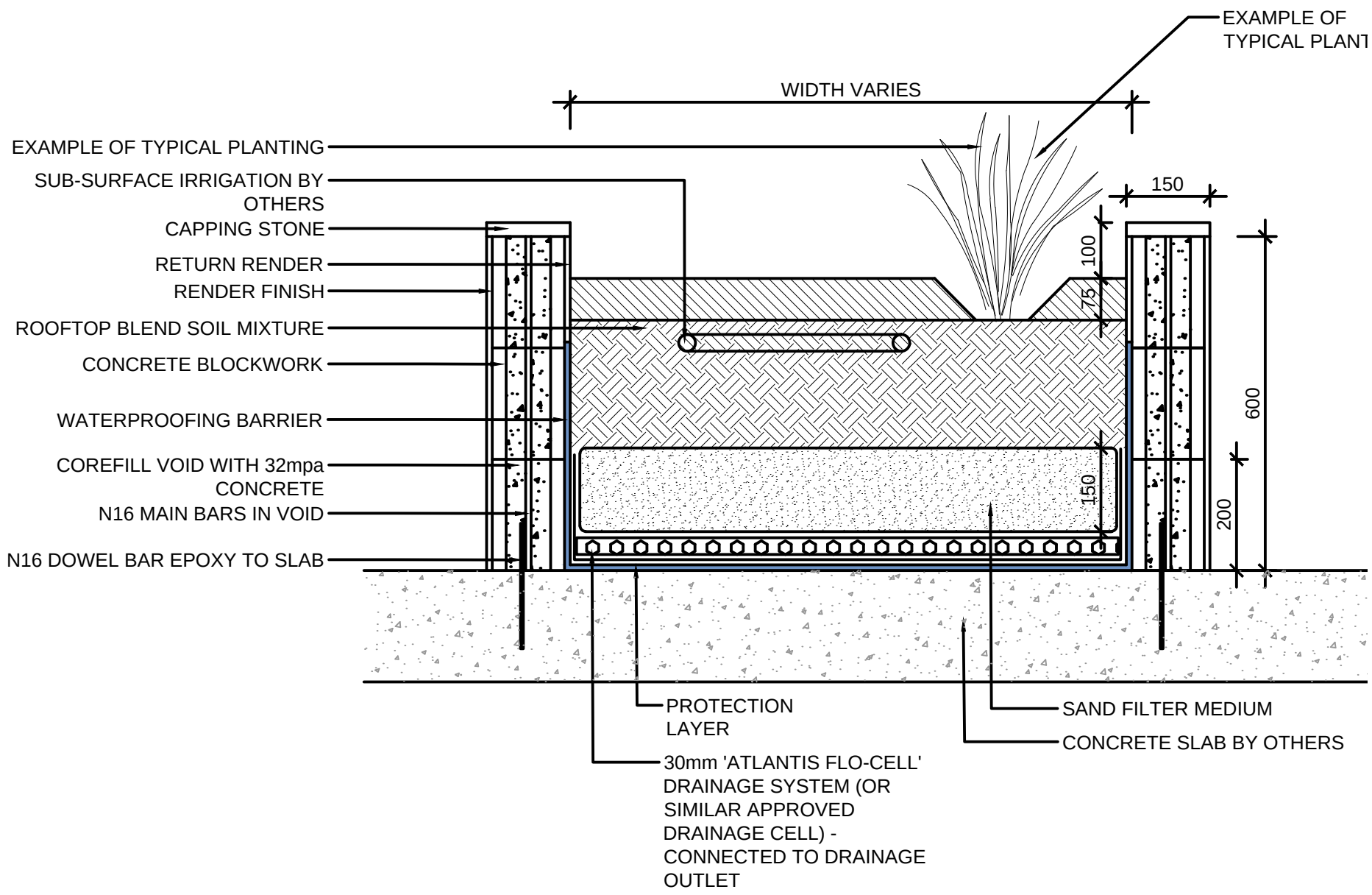
PLANTING IN ELEVATED PLANTER 1:10@A1
