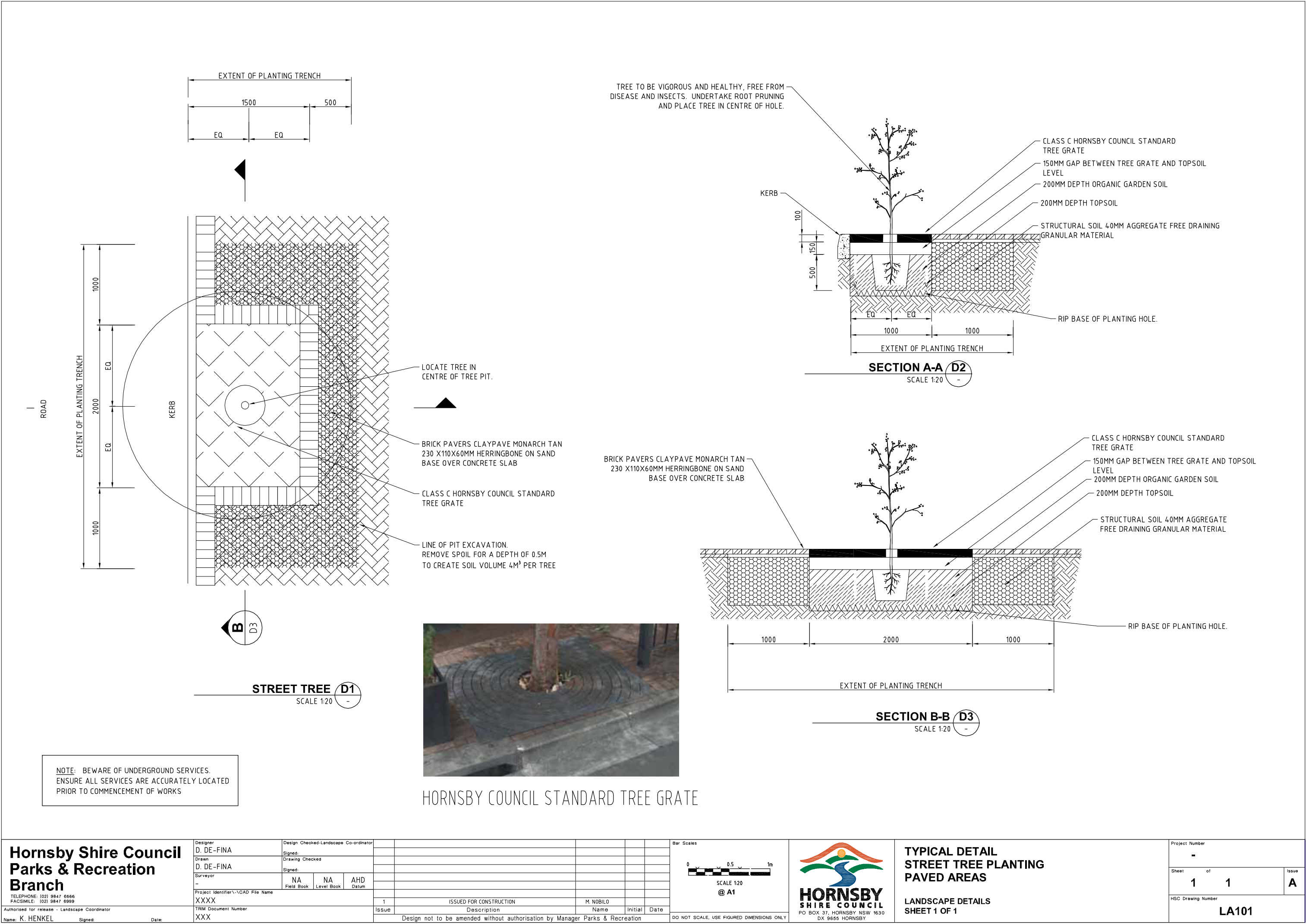
STREET TREE PLANTING TO HORNSBY COUNCIL STANDARDS AS PICTURED ABOVE
